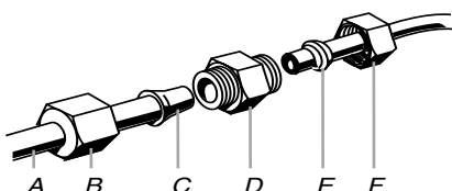
A. Water tubing B. Nut (provided) C. Bulb D. Coupling (purchased) E. Ferrule (purchased) F. Nut (purchased)
